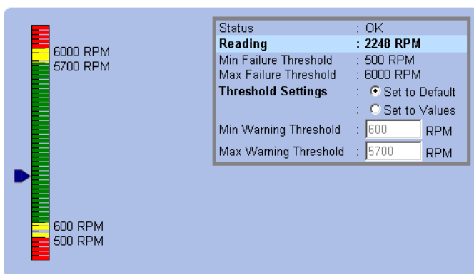
Figure 3-3. Gauge Indicator
